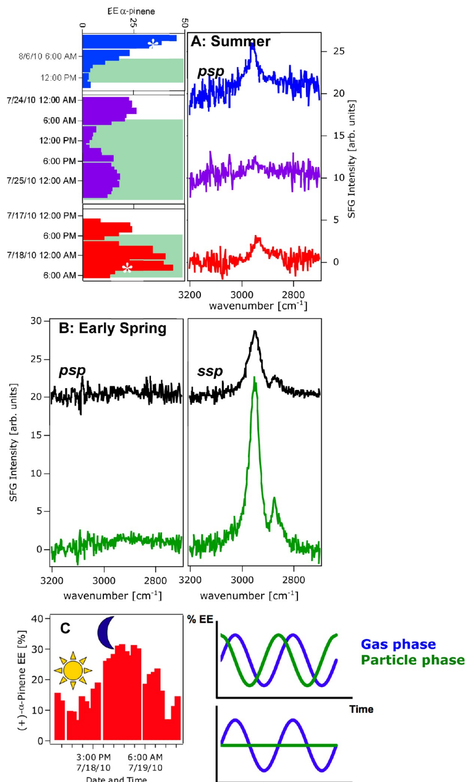
Figure 7. (A) Enantiomeric excess of (+)- \alpha -pinene in the gas phase and corresponding psp-polarized vibrational SFG spectra of aerosol particles collected in the PM1 size range during the times indicated in green, with asterisks marking high EE values associated with advection of emissions from the freshly sawn wood to the field measurement site. (B) psp-polarized (left) and ssp-polarized (right) SFG spectra obtained from particles collected on 23 (top) and 25 (bottom) March 2011. (C) (+)- \alpha -Pinene enantiomeric excess (EE) as a function of hour in the day of 18 to 19 July 2010 (left) and concept for a chiral carbon tracer to connect aerosol gas phase with aerosol particle phase chemistry (right). Please see text for details.
